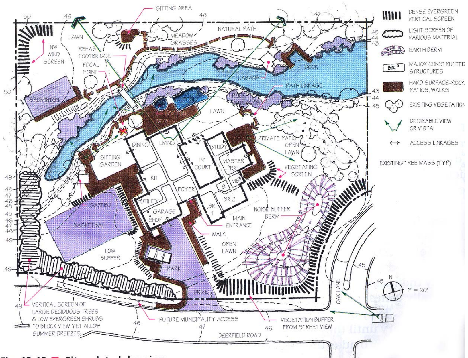
Fig. 13-13 ■ Site-related drawing.
