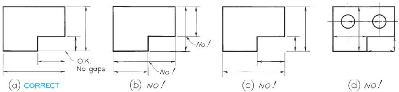
FIGURE 11.3 Dimension and Extension Lines.
