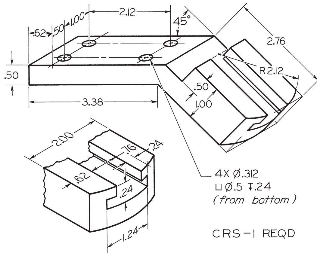
FIGURE 8.35 Guide Bracket.
