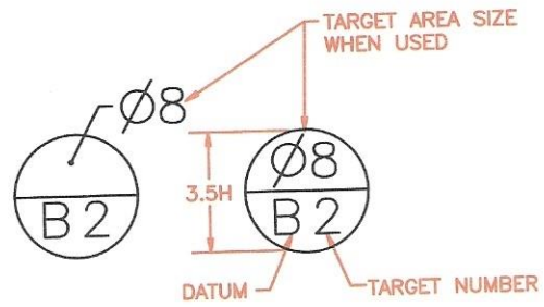
DATUM TARGET SYMBOL
