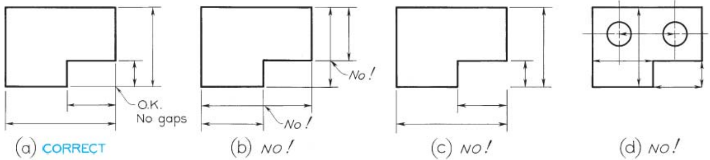
FIGURE 11.3 Dimension and Extension Lines.
