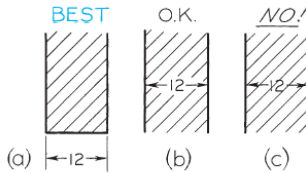
FIGURE 11.13 Dimensions and Section Lines. Metric.
