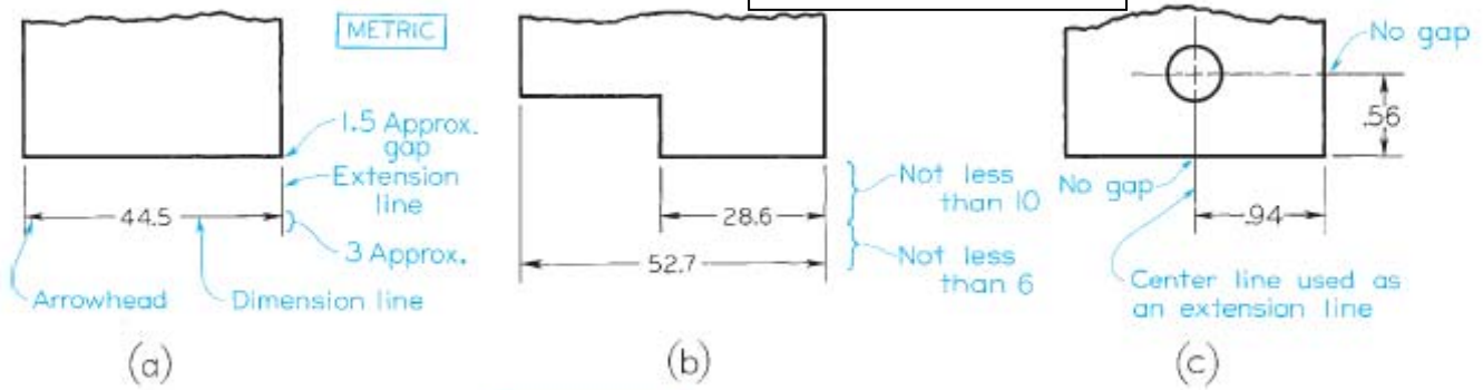
FIGURE 11.2 Dimensioning Technique.
