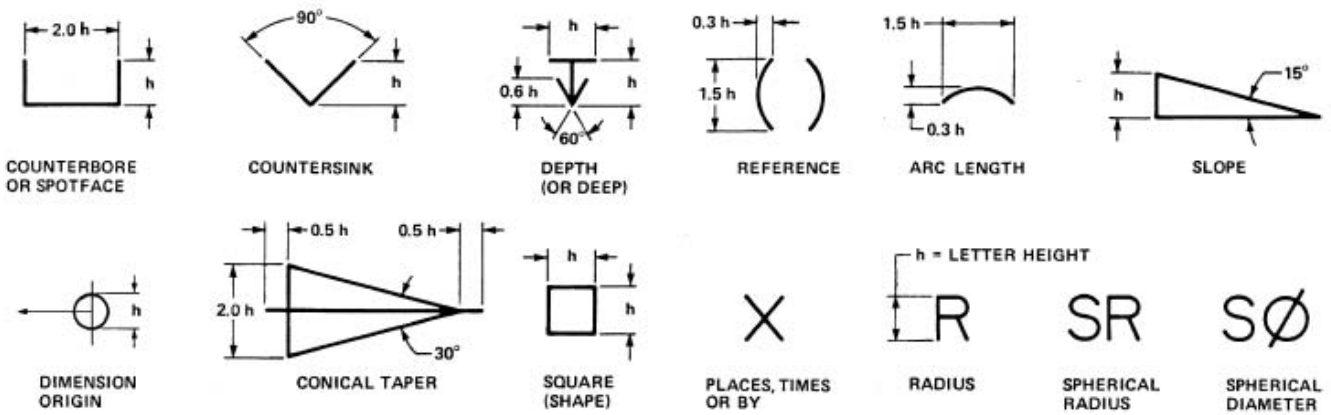
FIGURE 11.29 Form and Proportion of Dimensioning Symbols (ANSI/ASME Y14.5M-1994).
