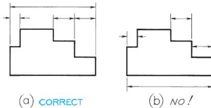
FIGURE 11.4 Grouped Dimensions.
