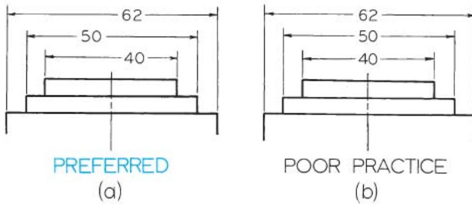
FIGURE 11.14 Staggered Numerals. Metric.
