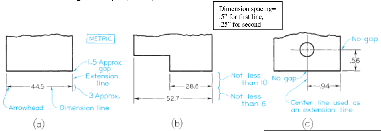
FIGURE 11.2 Dimensioning Technique.
