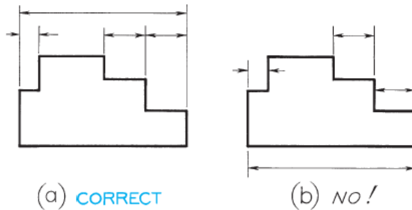
FIGURE 11.4 Grouped Dimensions.
