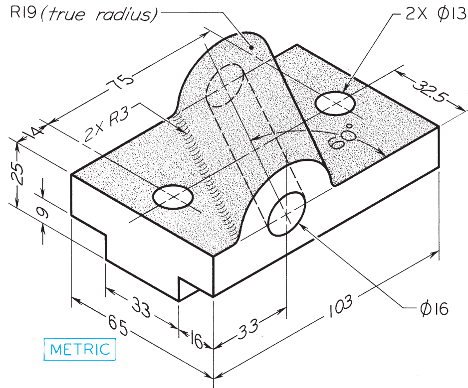
FIGURE 8.33 Guide Block.
